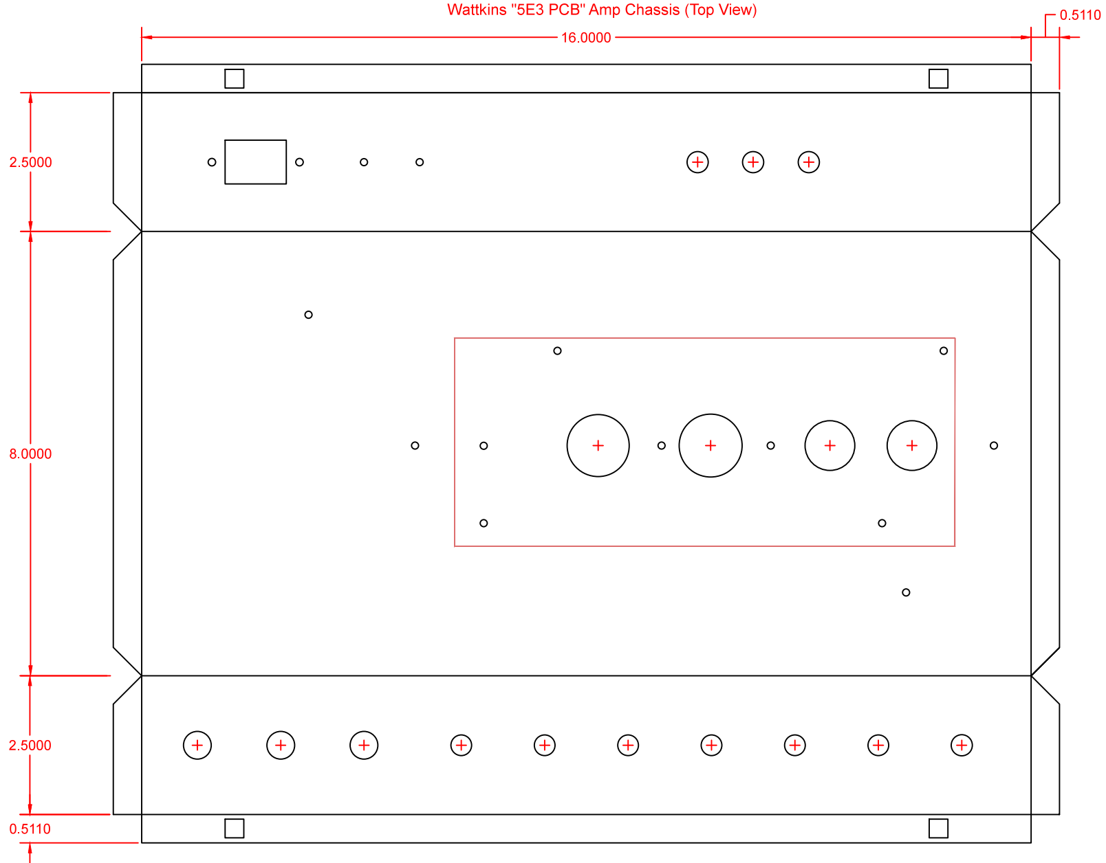
Watkins "5E3 PCB" Amp Chassis (Top View)
